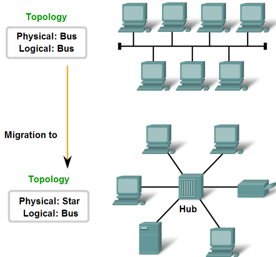
Early Ethernet Media and Topology
