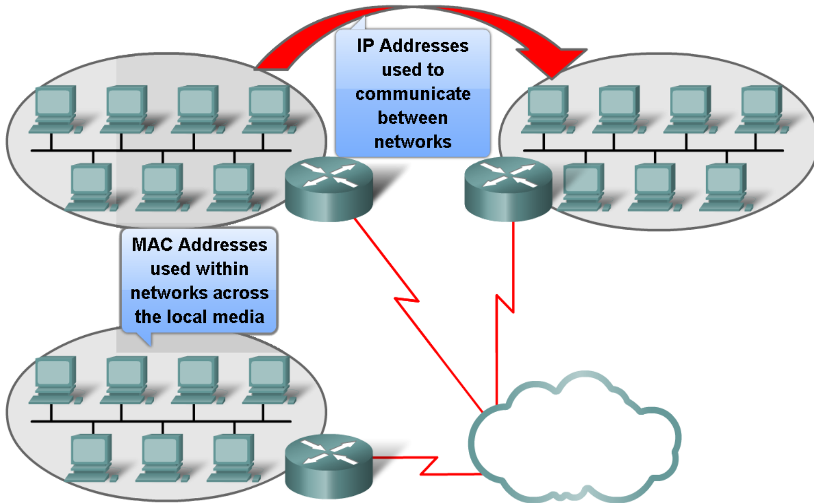
Different Layers of Addressing
